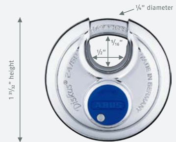
2" width 24IB/50
